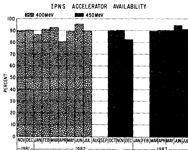
Fig. 2. IPNS accelerator availability since turn-on.
