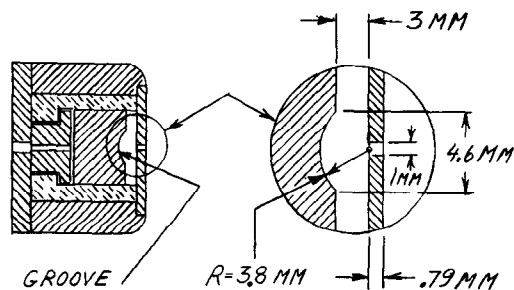
Fig. 3. Magnetron H^- ion source with grooved cathode.
