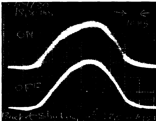
Fig. 4. IPNS beam bunch at 430 MeV. Upper trace - artificially diluted by synchrotron noise. Lower trace - undiluted.
