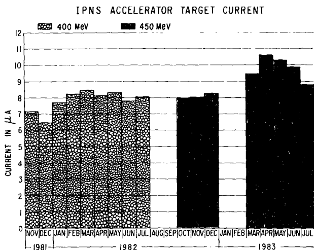
Fig. 1. IPNS Accelerator average target current.
