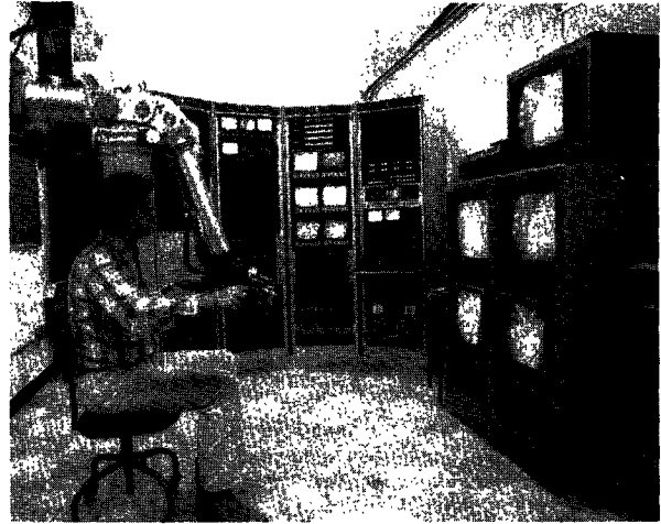
Fig. 3. Monitor Control Room
