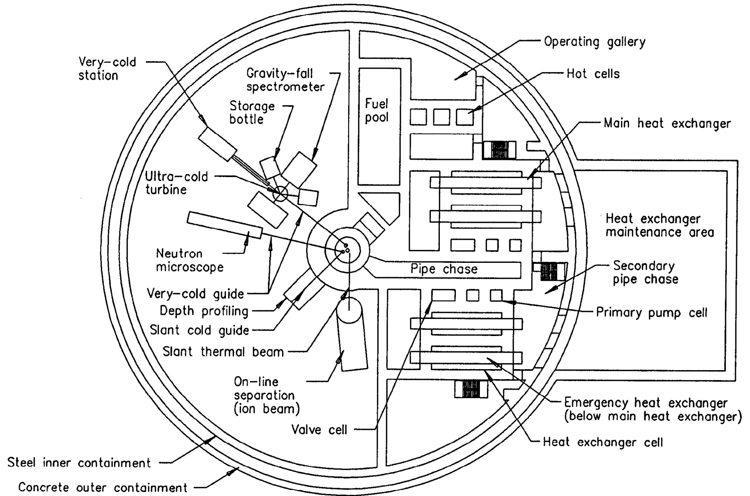
Figure 6. A possible arrangement of the Second Floor Beam Room.
