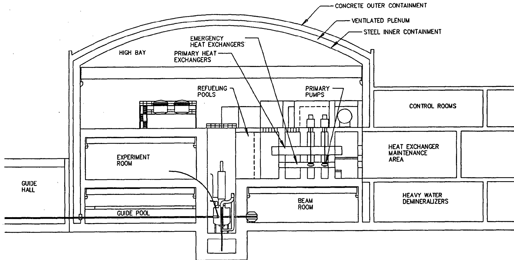
Figure 3. Vertical section through the ANS reactor building, showing experiment halls.
