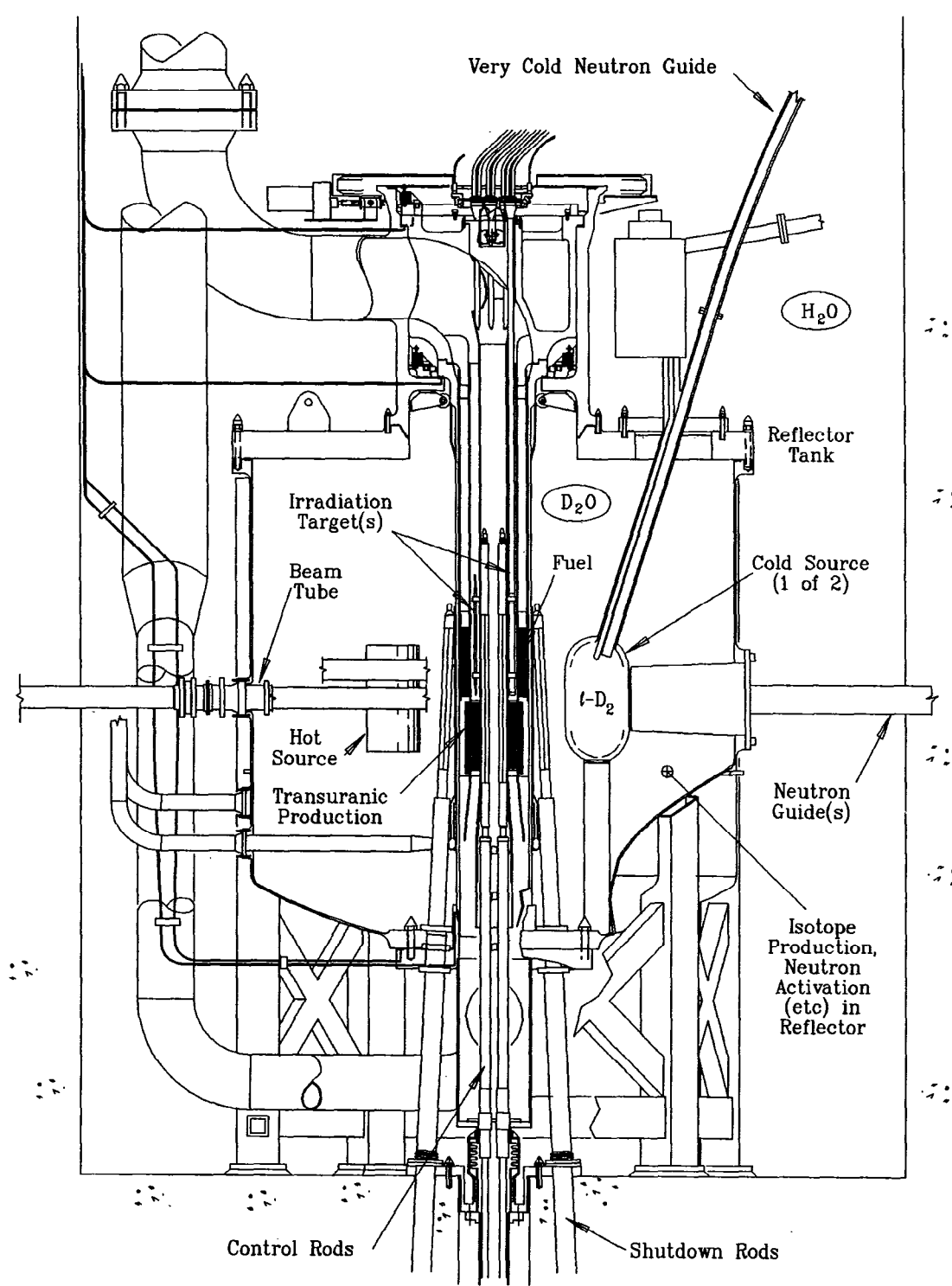
Figure 2. The ANS reactor assembly.
