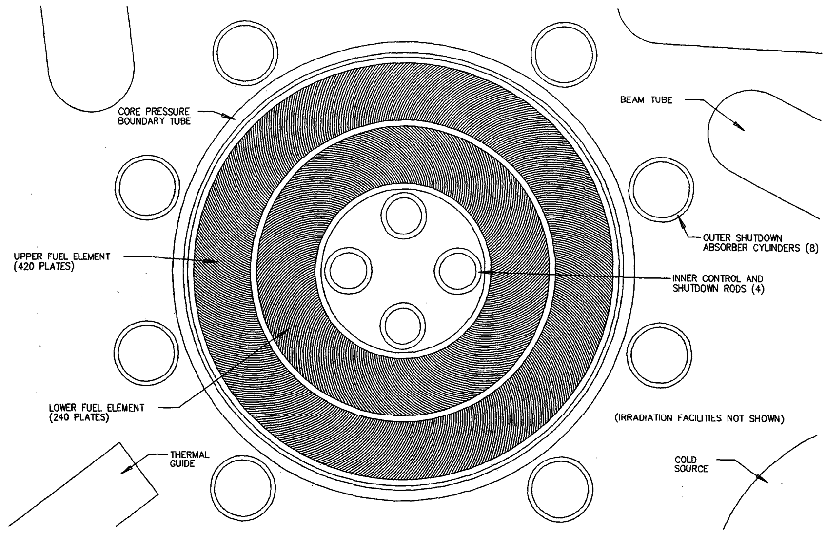
Figure 1. Plan view of the ANS reactor core.
