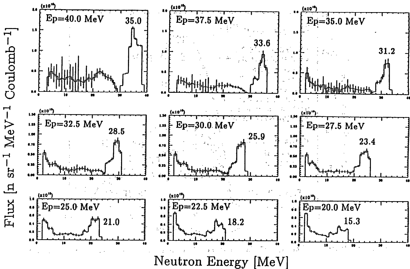
Fig. 1 Semi-monoenergetic neutron energy spectra for proton energies of 20, 22.5, 25, 27.5, 30, 32.5, 35, 37.5, 40 MeV
