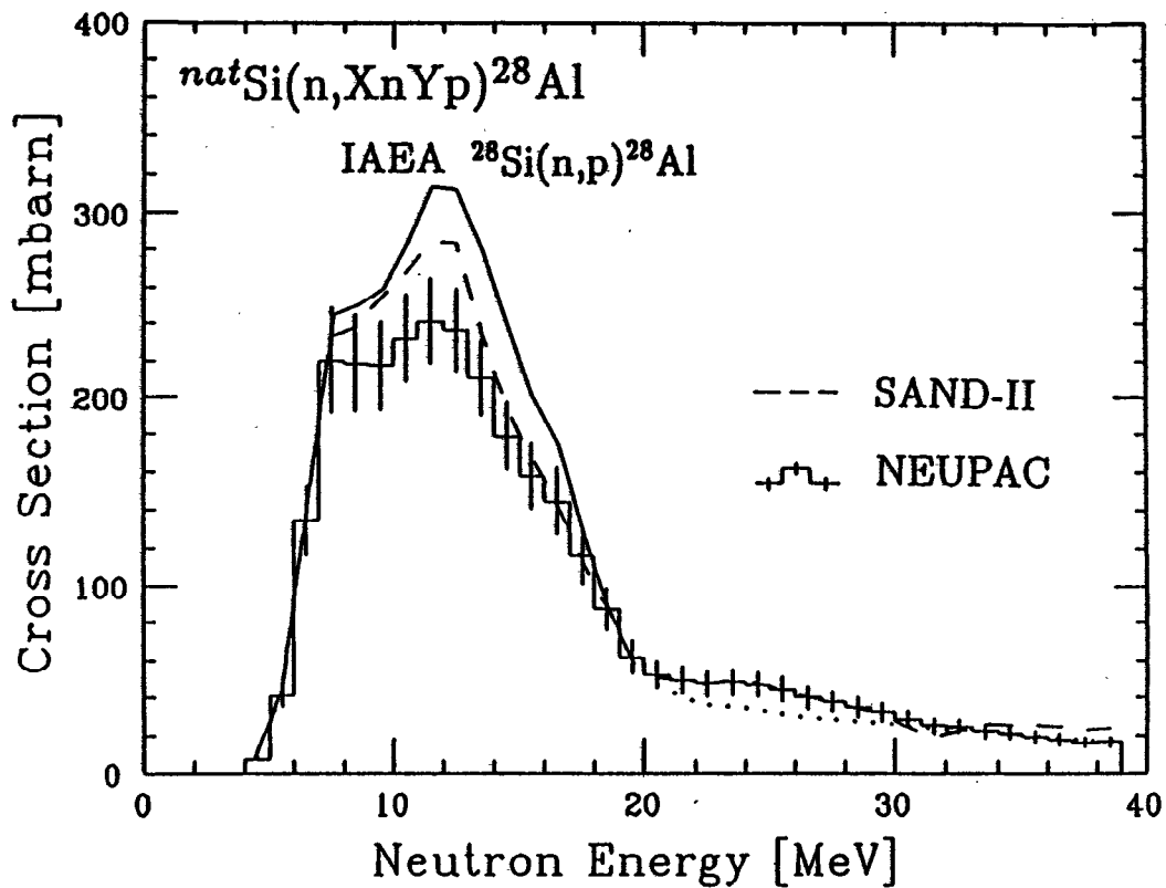
Fig. 5 Measured ^{nat}\text{Si}(n, XnYp)^{28}\text{Al} cross section data, together with the cited data
