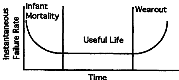
Fig. 1 Bathtub Curve
