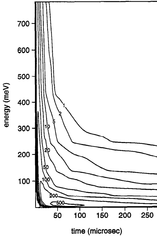
Figure 6. Contour plot of brightness as a function of time and energy for the 60-cm Be/Pb case. The units on the contour values are 10^{15} n/cm 2 /s/sr/eV/s/MW.
