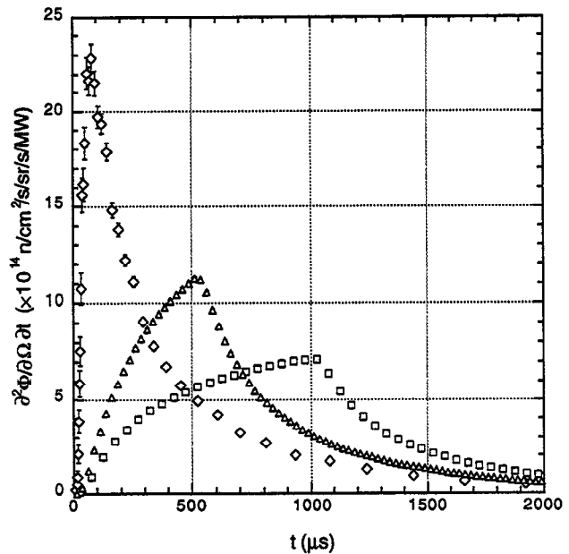
Figure 5. Pulse shapes ( E < 5 meV) for the 60-cm Be/Pb case for three proton pulse widths: ( \diamond ) instantaneous; ( \blacktriangle ) 0.5 ms; ( \blacksquare ) 1 ms.
