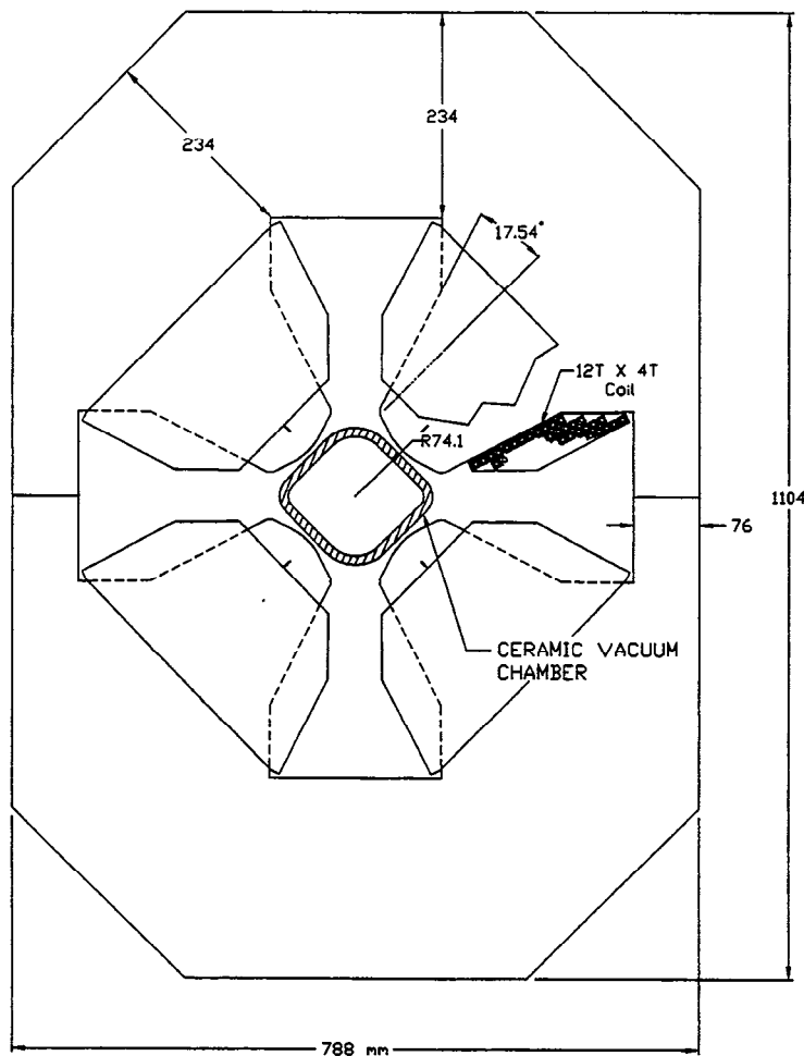
Figure 9: End View of a Synchrotron Quadrupole Magnet.
