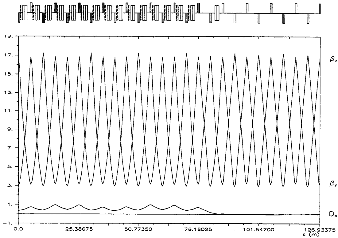
Figure 2: Lattice Functions for 1/2 Super-Period.
