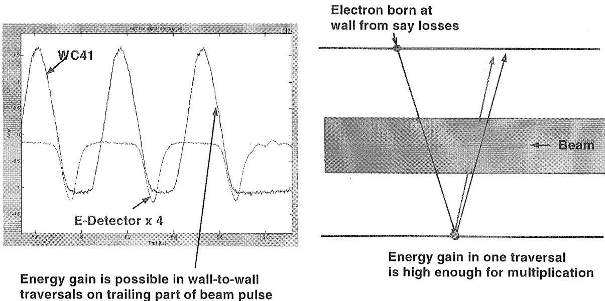
Figure 7. Schematic description of the "trailing edge multipactor" mechanism.
