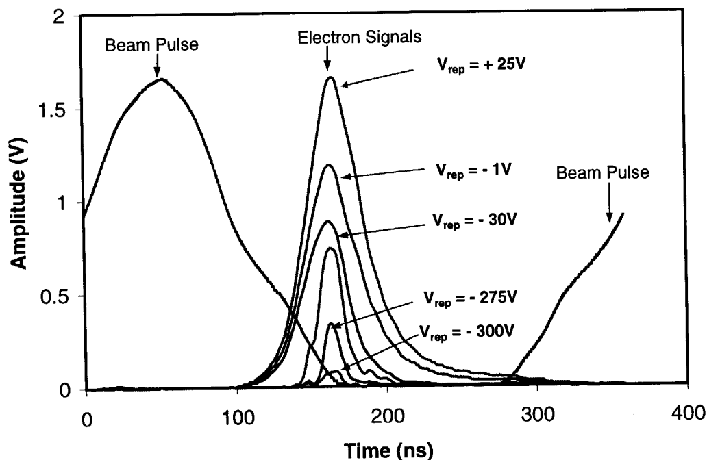
Figure 3. Electron signals during a single revolution in the ring shown in proper time relation to the beam signal (wall current monitor).
