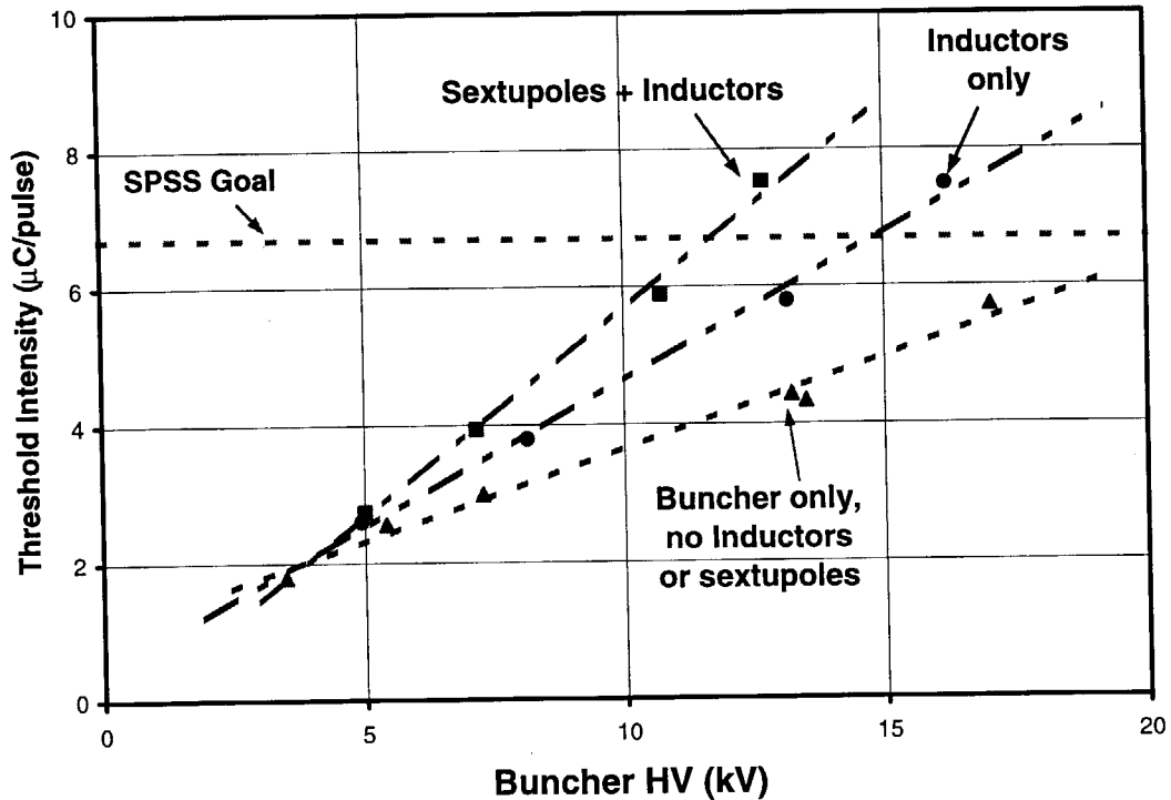
Figure 1. Effect of inductive inserts and sextupoles on the instability threshold-intensity curves.
