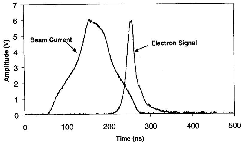
Figure 8. Electron signal in relation to a 6.8 \mu\text{C} beam pulse in a single pass experiment.
