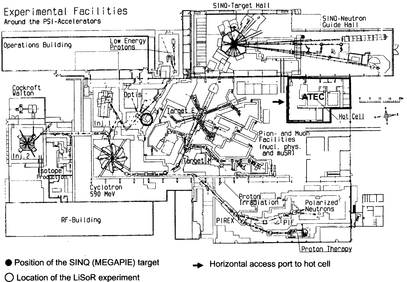
Figure 2: Schematic floor plan of the PSI accelerator complex and associated research facilities
