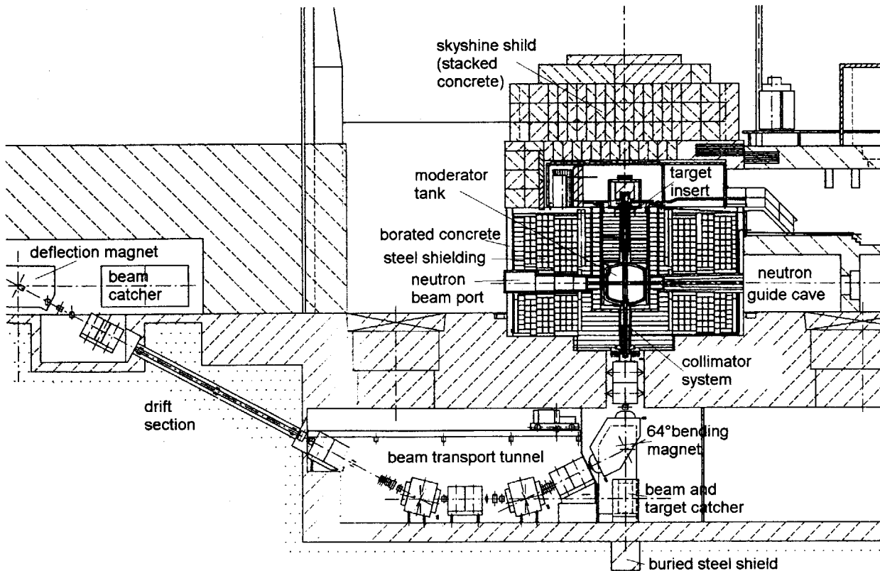
Figure 2: Vertical cut through the target block and part of the proton beam transport line of SINQ
