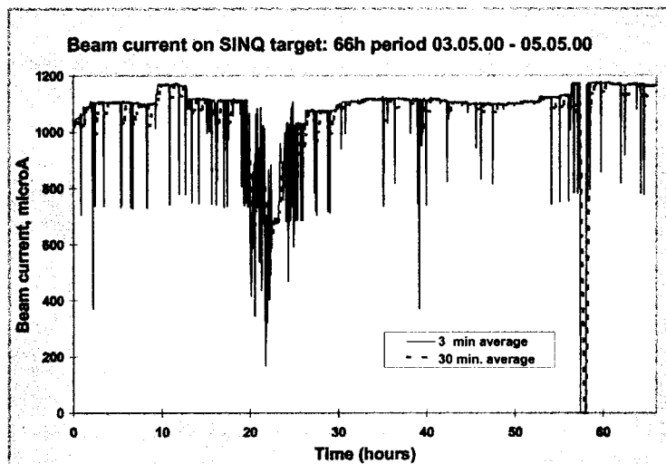
Figure 6: Example of beam stability problems the MEGAPIE target will have to cope with. Solid line: 3 min average; dashed line: 30 min. average
