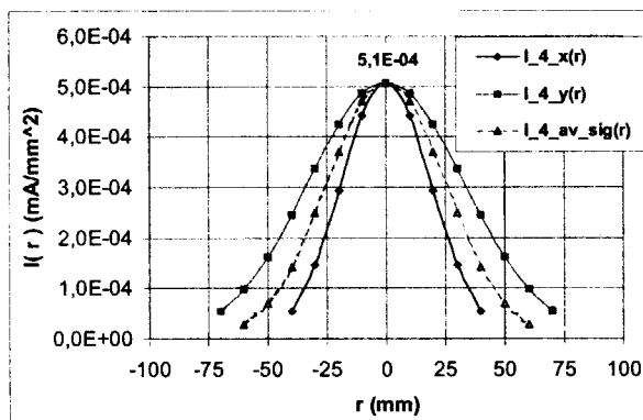
Figure 5: Reference beam intensity distribution for the design of the 1 MW MEGAPIE target ( I_{SINQ} = 1.74 \text{ mA} at 575 MeV)
