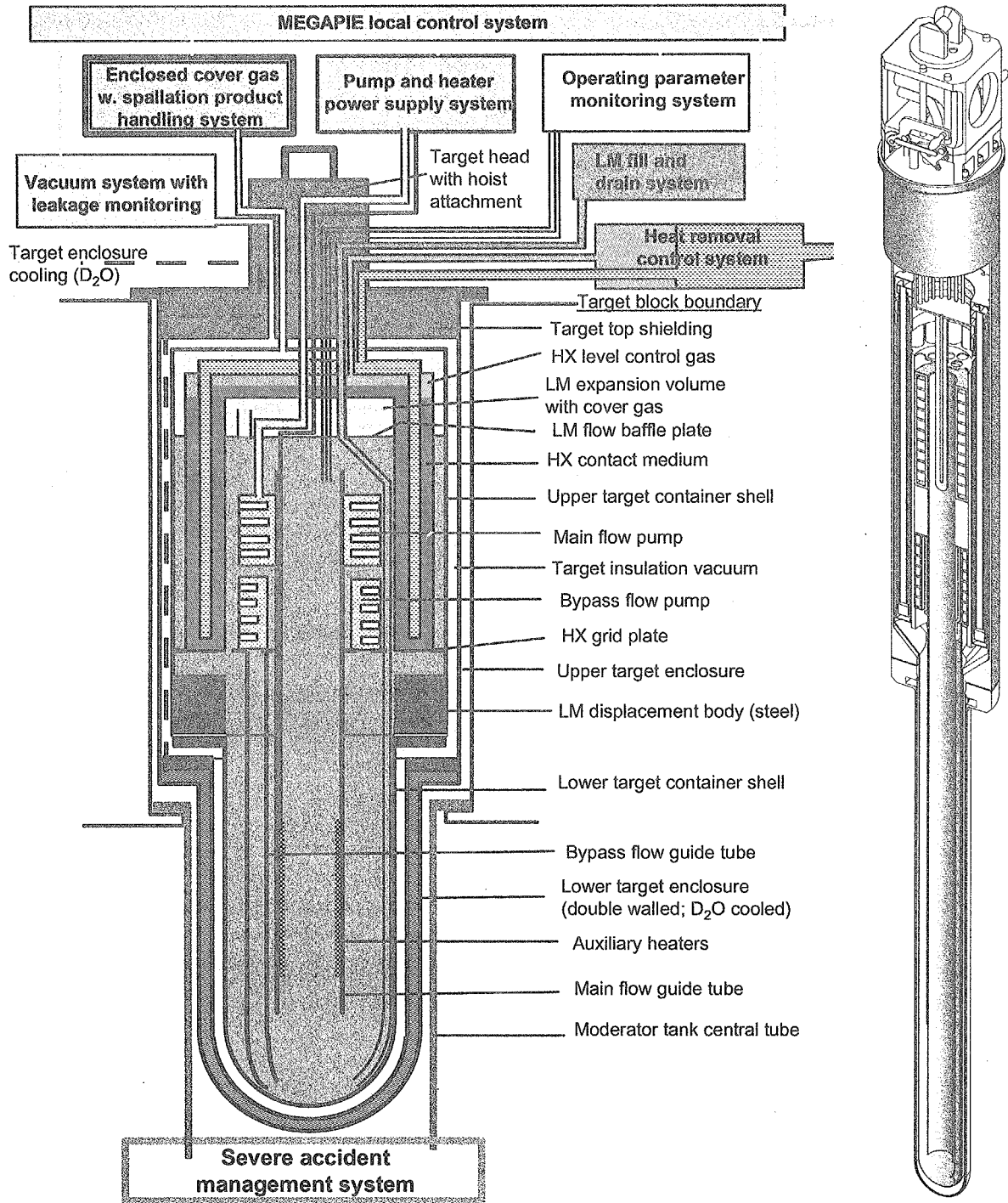
Fig. 7 The basic concept (left) and conceptual design (right) of the MEGAPIE target
