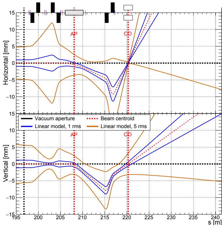
Figure 1: The transverse beam sizes along the beam delivery line from the accelerator to the target (far right edge of plot) at maximum raster amplitudes. The location and polarity of 6 DC quadrupoles are represented by black boxes.
