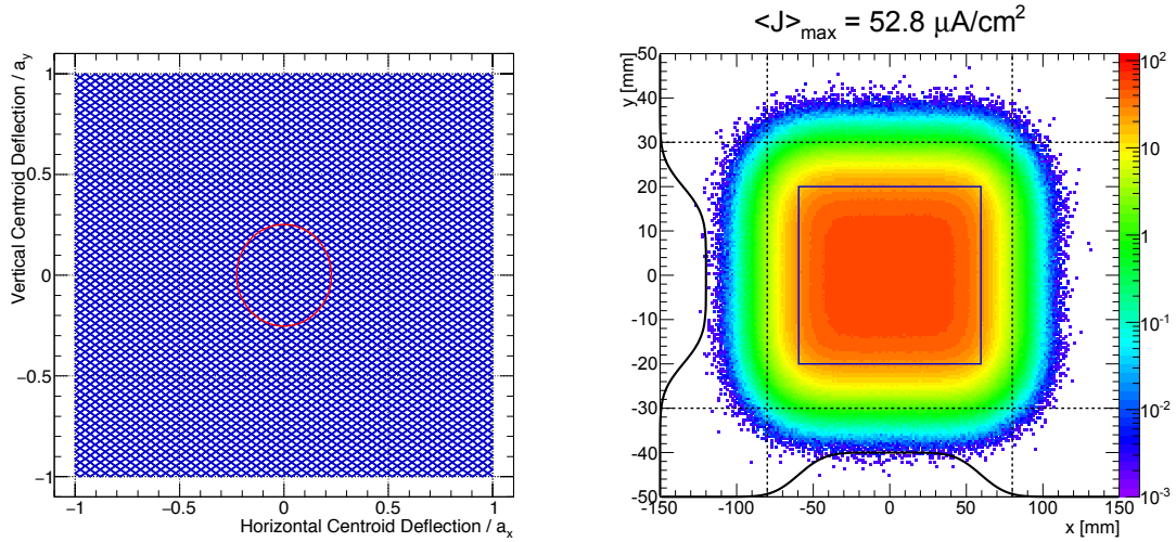
(a) A Lissajous-pattern generated by triangle waveforms with a frequency ratio of 113/83. For comparison, the beamlet relative RMS sizes at the target are illustrated by a red ellipse.
