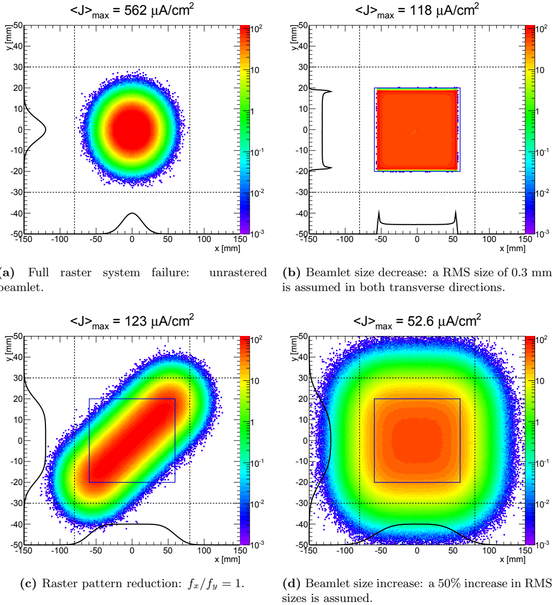
Figure 5: Simulation results similar to Fig. 2b but including beam delivery system failures that result in errant beam conditions.
