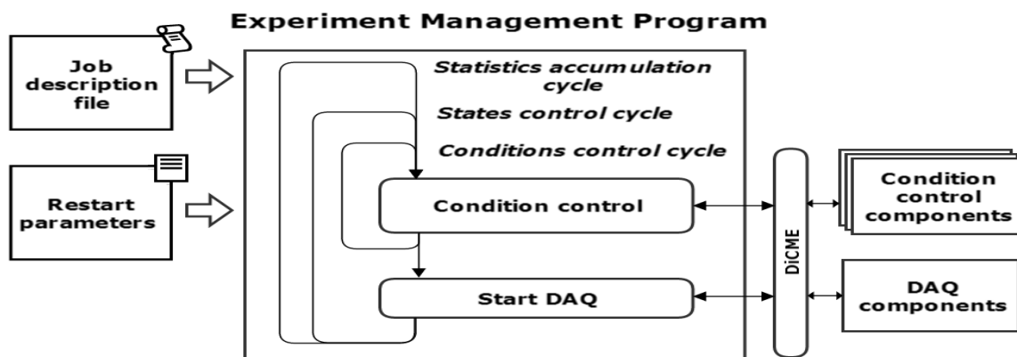
Figure 5. Scheme of the experiment management program for long measurements.
