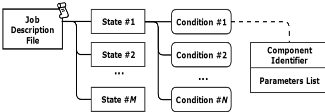
Figure 1. The structure of the PSJ file for an experiment
